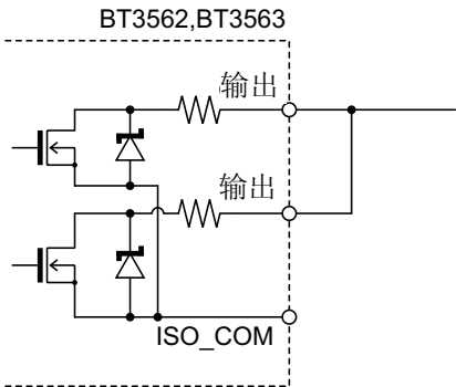
Wired OR
